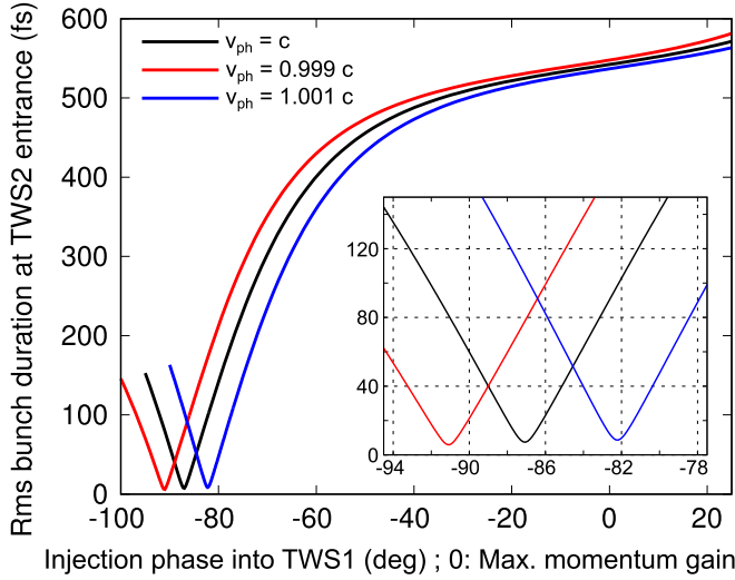
FIG. 3. Simulated rms bunch duration after TWS1 as a function of the injection phase into it for several phase velocities v_{ph} . The inset shows a zoom around the maximal compression. Conditions: 1 pC charge; 320 \mu\text{m} transverse diameter of laser pulse driving the gun; 74 MV/m gun peak accelerating field (RF-gun at the phase maximizing the momentum \rightarrow 3.85 MeV/c output bunch); See Table II.
