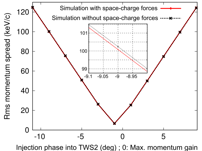
FIG. 2. ASTRA simulation of the bunch rms momentum spread at the high-energy spectrometer as a function of the injection phase into TWS2. The inset shows a zoom around one TWS2 phase. Conditions: 1 pC charge; 320 \mu\text{m} transverse diameter of laser pulse driving the gun; 74 MV/m gun peak accelerating field (RF-gun at the phase maximizing the momentum \rightarrow 3.85 MeV/c output bunch); TWS1 at the phase maximizing the momentum \rightarrow 78.5 MeV/c output bunch; 542.24 fs rms bunch duration at TWS2 entrance; See Table II. Note: The with or without space-charge forces refers only to the path into TWS2, the simulation up to TWS2 entrance is with space-charge forces.
