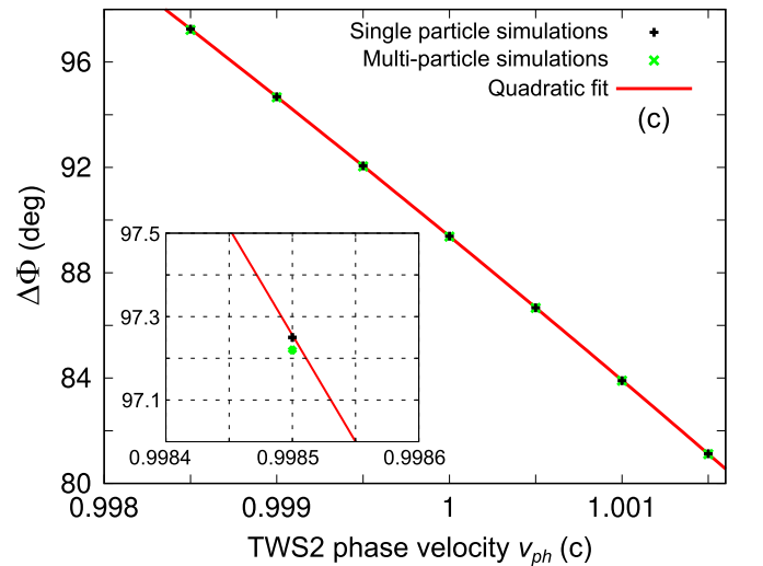
FIG. 4. (a): Simulated average momentum after TWS1 as a function of the injection phase into it for several phase velocities v_{ph} . Phase gap \Delta\Phi between the maximum momentum and saddle point as a function of v_{ph} for TWS1 (b) and TWS2 (c). Conditions: Single particle and multi-particle simulations; See caption of Fig. 5; See Table II.
