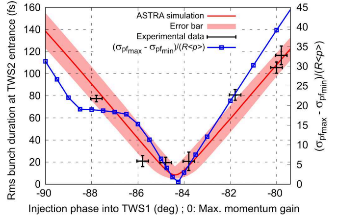
FIG. 11. Rms bunch duration at TWS2 entrance and (\sigma_{p_{f_{max}}} - \sigma_{p_{f_{min}}}) / (R \langle p \rangle) as a function of the injection phase into TWS1 ( 0^\circ \equiv max. momentum gain). The variable (\sigma_{p_{f_{max}}} - \sigma_{p_{f_{min}}}) / (R \langle p \rangle) is used to check the applicability of the phase scan method (see Sec. III B). Conditions: See Fig. 9 (c).
