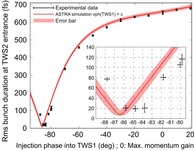
FIG. 10. Rms bunch duration at TWS2 entrance as a function of the injection phase into TWS1 ( 0^\circ \equiv max. momentum gain). The phase velocity of TWS1 is here set to c (the design value) in the ASTRA simulation, instead of the experimentally measured value ( 1.00040 c ) as in Fig. 9 (c). Conditions: See Fig. 9 (c).
