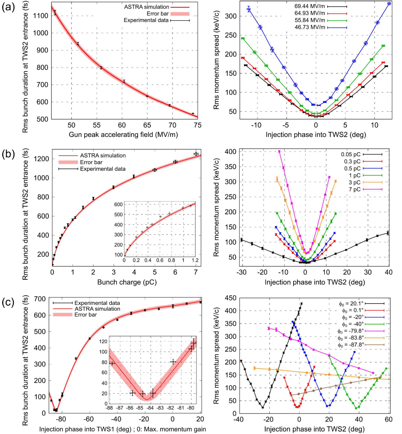
FIG. 9. Rms bunch duration at TWS2 entrance as a function of the RF-gun peak accelerating field (a), the bunch charge (b) and the injection phase into TWS1 (c). 0^\circ \equiv max. momentum gain. Aside of each duration curve, a selection of the raw data used for the measurements is displayed. Conditions: Mo (a,b) and \text{Cs}_2\text{Te} (c) cathode; 320 \mu\text{m} (a,c) and 800 \mu\text{m} (b) transverse diameter of laser pulse driving the RF-gun; 64.9 \text{ MV/m} (b) and 69.5 \text{ MV/m} (c) gun peak accelerating field (resp. 3.43 and 3.64 \text{ MeV/c} output momentum); (1.08 \text{ to } 1.05 \pm 0.02) \text{ pC} depending on point (a) and (1.27 \pm 0.02) \text{ pC} before collimator and (1.01 \pm 0.02) \text{ pC} after collimator (c); Injection phases into RF-gun adjusted to maximize the momentum (except for the points at 46.7 \text{ MV/m} (resp. 51.3 \text{ MV/m} ) in (a) where it is fixed to +6.7^\circ (resp. +11.7^\circ ) above the zero-crossing field); Injection phase into TWS1 adjusted to maximize the momentum gain (a,b); See Table II. Note: For (b), the error bars on the charge for the 3 highest points are larger because of a different setting of the Faraday Cup. The charge for the lowest point ( 0.015 \text{ pC} ) has not been directly measured with the Faraday Cup but extrapolated from the cathode laser settings.
