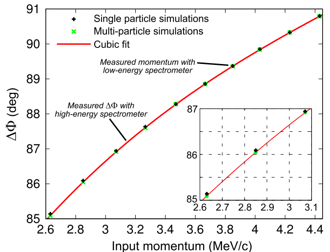
FIG. 6. Phase gap \Delta\Phi between the maximum momentum and saddle point at the exit of TWS1 as a function of the input bunch momentum. Conditions: Single particle and multi-particle ( 10^4 macroparticles including space-charge forces) ASTRA simulation; RF-gun at the phase maximizing the momentum (field amplitude is varied to change the bunch momentum); v_{ph} (TWS1) assumed equal to c (the design value); See caption of Fig. 5 (a) and Table II.
