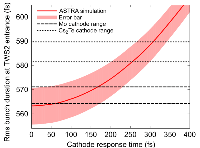
FIG. 8. Rms bunch duration at TWS2 entrance as a function of the cathode response time simulated by ASTRA compared with the experimental values measured for a Mo and a Cs 2 Te cathode with their uncertainty ranges. The error bar on the ASTRA simulation has been computed by including the jitter on the bunch charge, an uncertainty of \pm 0.25 A on the current injected into the focusing solenoid located after the RF-gun and the uncertainty on TWS1 phase velocity. Conditions: See Fig. 7 caption.
