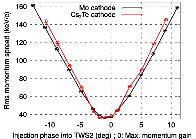
FIG. 7. Raw data for bunch duration determination at TWS2 entrance (rms momentum spread as a function of injection phase) for Mo and Cs 2 Te cathodes in identical conditions. Conditions: (1.07 \pm 0.015) pC charge; 320 \mu\text{m} transverse diameter of laser pulse driving the gun; 70.6 MV/m gun peak accelerating field ( 3.69 MeV/c output momentum); Injection phases into RF-gun and TWS1 adjusted to maximize the momentum; See Table II.
