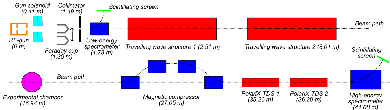
FIG. 1. Schematic layout of the ARES linac at DESY [6, 7] with the relevant elements for the study presented in this paper. The positions are given relative to the RF-gun cathode plane and at the entrance of each element.
