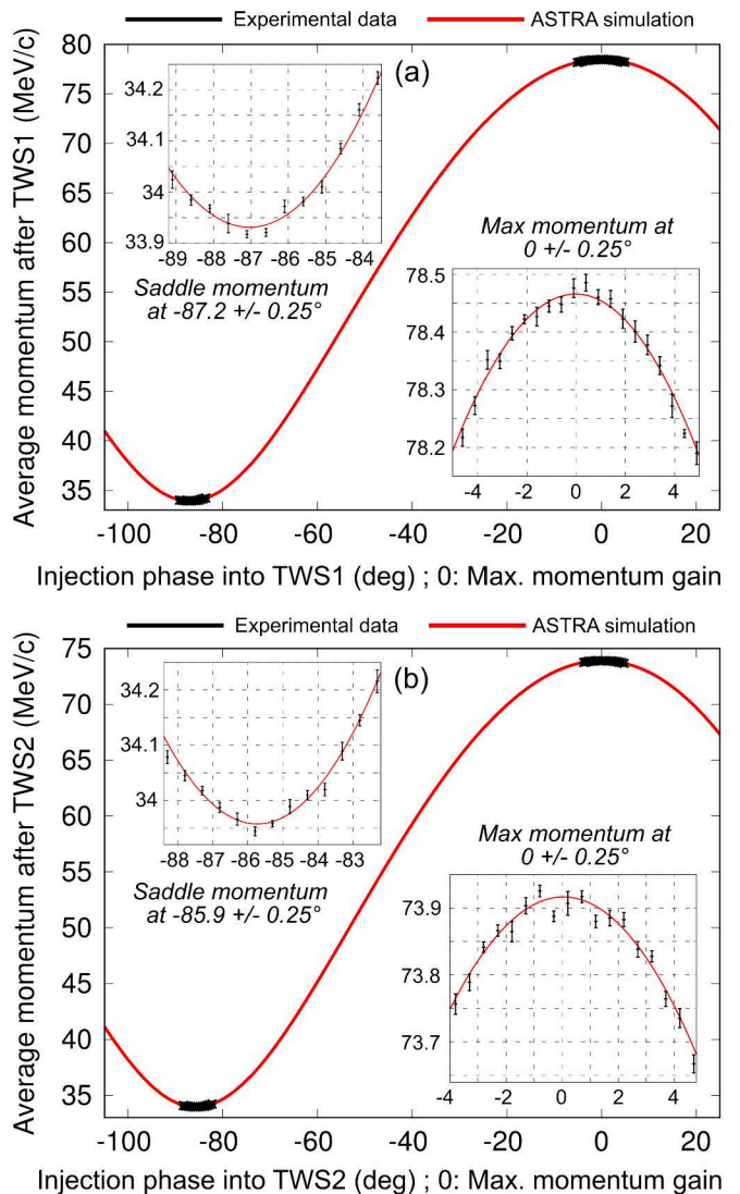
FIG. 5. Raw data for experimental determination of TWS1 (a) and TWS2 (b) phase velocities (average momentum as a function of injection phase). The insets show zooms around the maximum and saddle momentum phase ranges. Conditions: Mo cathode; 0.9 pC (a) and 0.25 pC (b) charge; 320 \mu\text{m} transverse diameter of laser pulse driving the gun; 74 \text{ MV/m} gun peak accelerating field (RF-gun at the phase maximizing the momentum \rightarrow 3.85 \text{ MeV/c} output particle); TWS2 off (a); TWS1 off (b); See Table II.
